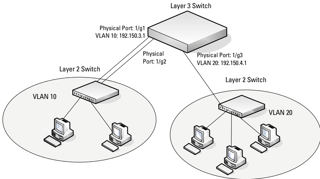
Figure 4-1. VLAN Routing Example Network Diagram
